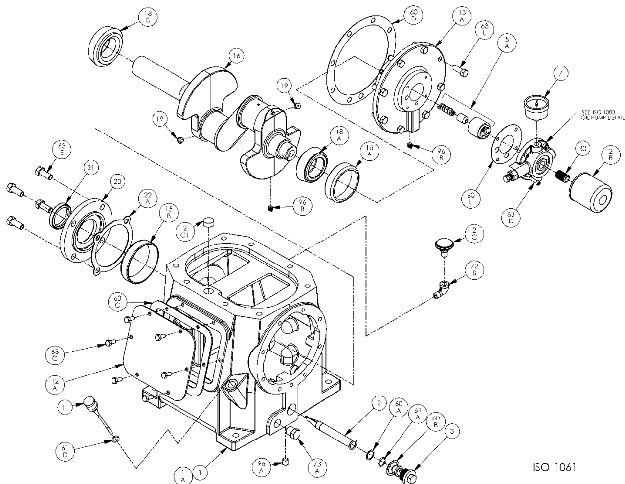
Crankcase ISO1061
